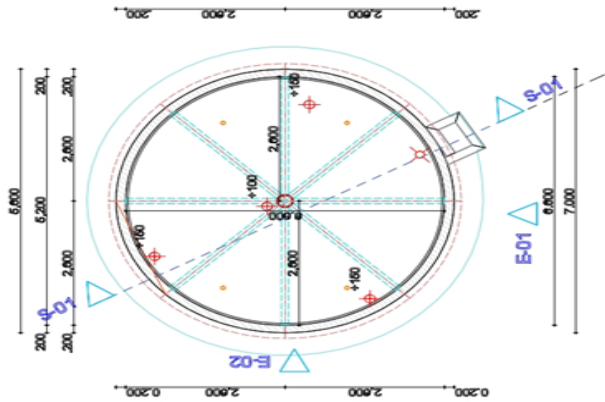
GROUND FLOOR LAYOUT
