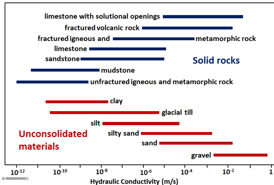
Figure 2.1: Hydraulic conductivities of various rocks.
